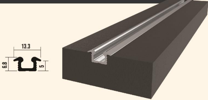
3010 R / GÖMME RAY
