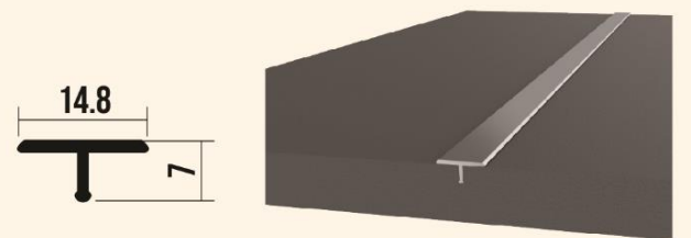
5050 S / İNCE T PROFİL
