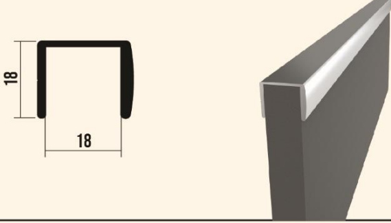
5594 S / 18 MM U
